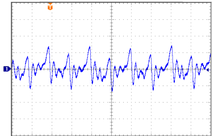
Figure 14: Input Terminal Ripple Current, i_c , at full rated output current and nominal input voltage with 4.7\mu H source impedance and 470\mu F electrolytic capacitor (Ch.1 500mA/div). (See Figure 13).
