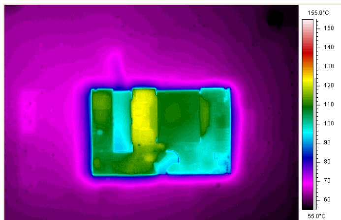
Figure 6: Thermal Image of converter at 4.8 amp load current (240W) with 55°C air flowing at the rate of 200 LFM. Air is flowing from pin 3 to pin 1 (nominal input voltage).
