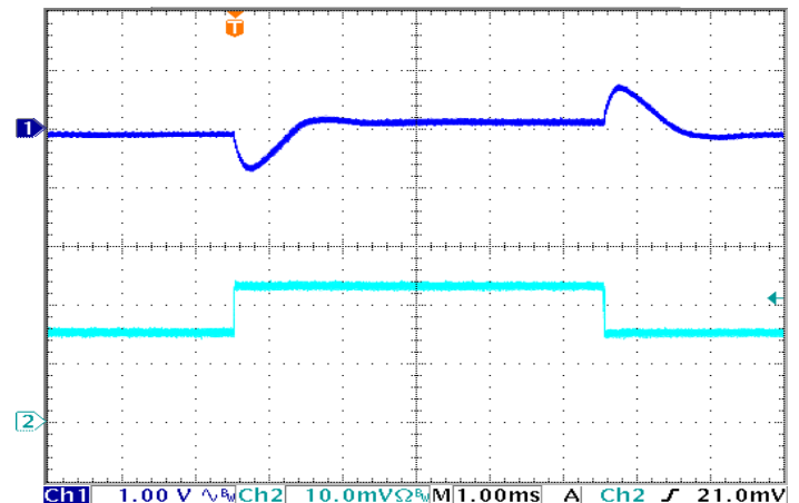
Figure 12: Output Voltage Response to Step-Change in Load Current (50%-75%-50% of I_{out(max)} ; dI/dt = 1A/\mu s ). Load cap: 330 \mu F electrolytic output capacitance. Top trace: Vout (1V/div). Bottom trace: Iout (2A/div).
