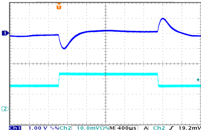
Figure 11: Output Voltage Response to Step-Change in Load Current (50%-75%-50% of I_{out(max)} ; dI/dt = 0.1A/\mu s ). Load cap: 100 \mu F electrolytic output capacitance. Top trace: Vout (1V/div). Bottom trace: Iout (2A/div).
