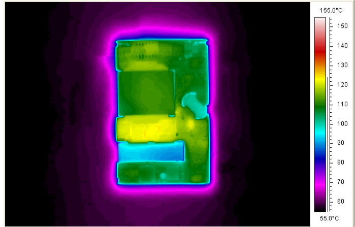
Figure 8: Thermal Image of converter at 4.6 amp load current (230W) with 55°C air flowing at the rate of 200 LFM. Air is flowing across the converter from input to output (nominal input voltage).
