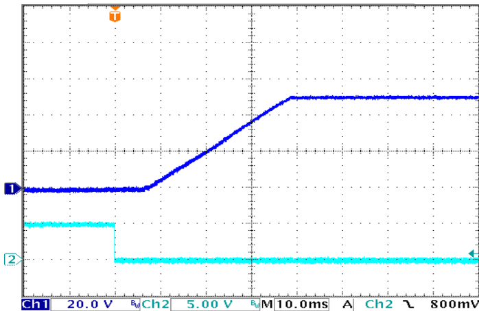
Figure 9: Turn-on Transient at full load (resistive load) (10 ms/div). Input voltage pre-applied. Top Trace: Vout (20V/div). Bottom Trace: ON/OFF input (5V/div)
