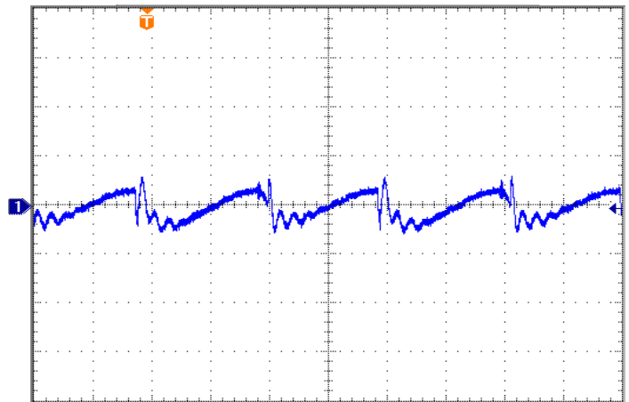
Figure 16: Output Ripple at nominal input voltage and rated load current (100 mV/div). Load capacitance: one 1.0\mu F ceramic capacitor and one 100\mu F electrolytic capacitor. Bandwidth: 20 MHz. (See Figure 13).
