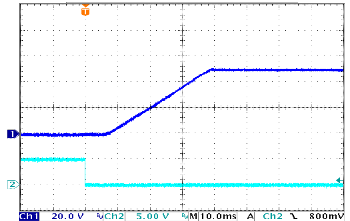
Figure 10: Turn-on Transient at zero load (10 ms/div). Top Trace: Vout (20V/div). Bottom Trace: ON/OFF input (5V/div)
